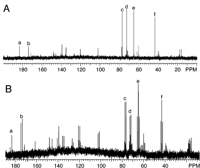
FIGURE 6: (A) ^{13}\text{C}\{^1\text{H}\} NMR spectrum (150 MHz) of a 3-DG + PM reaction mixture after 30 days at 37 °C. Signals a and c–f are attributed to the major reaction product. Chemical shifts are given in Table 1. The signal at ~102 ppm may be due to pyridoxal hydrate. (B) ^1\text{H} -coupled ^{13}\text{C} NMR spectrum of the same 3-DG + PM reaction mixture analyzed in (A). Multiplicities of the major signals are given in Table 1.
